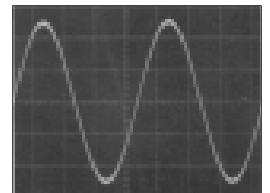
Photo (C) PS-500V output waveform (distortion approx. 0.2%)
