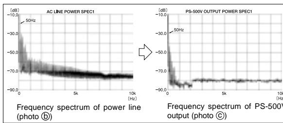
Frequency spectrum of power line
