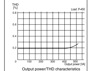
Fig. 2 PS-500V Load Characteristics
